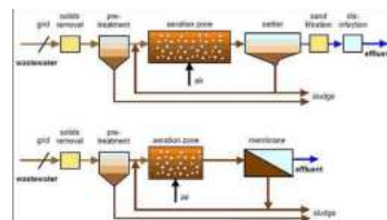
Figure 1: Membrane Bioreactor
