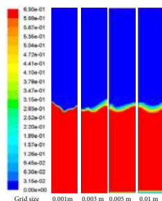
Figure 3: Contours of volume fraction of solids in Fluidized
